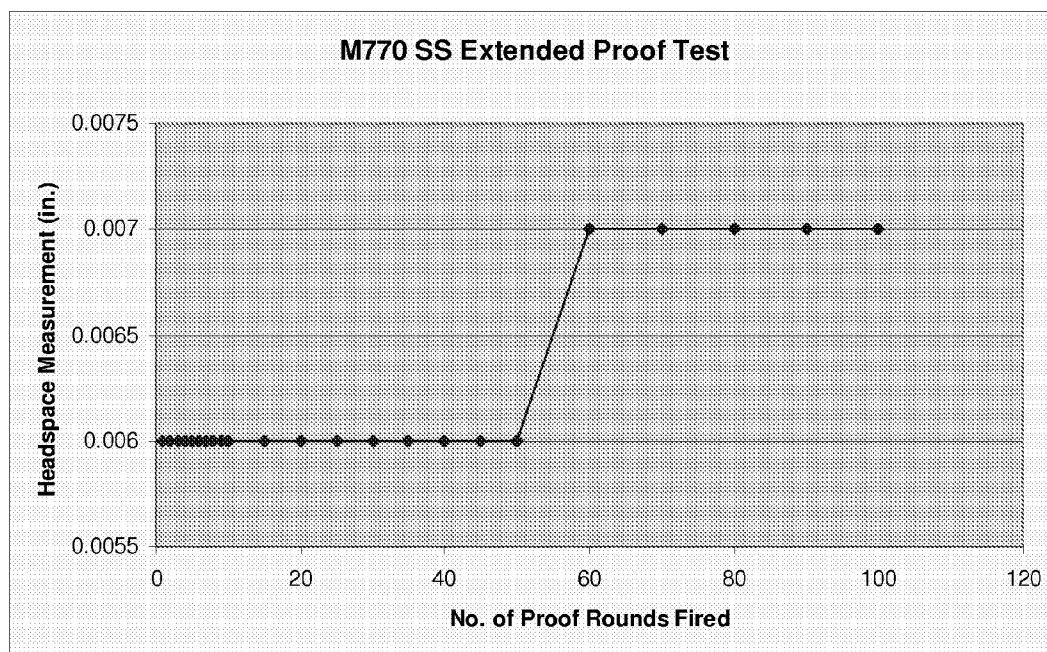
Figure 1: Headspace growth during Extended Proof of gun A7.
