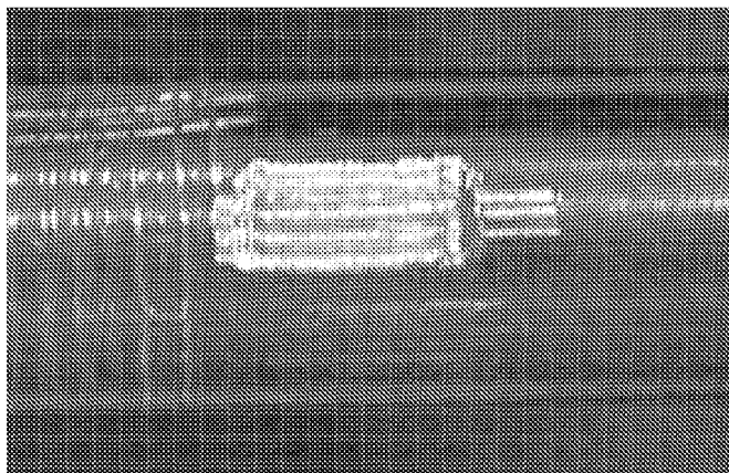
Figure 4: Gouged firing pin from gun A3.
