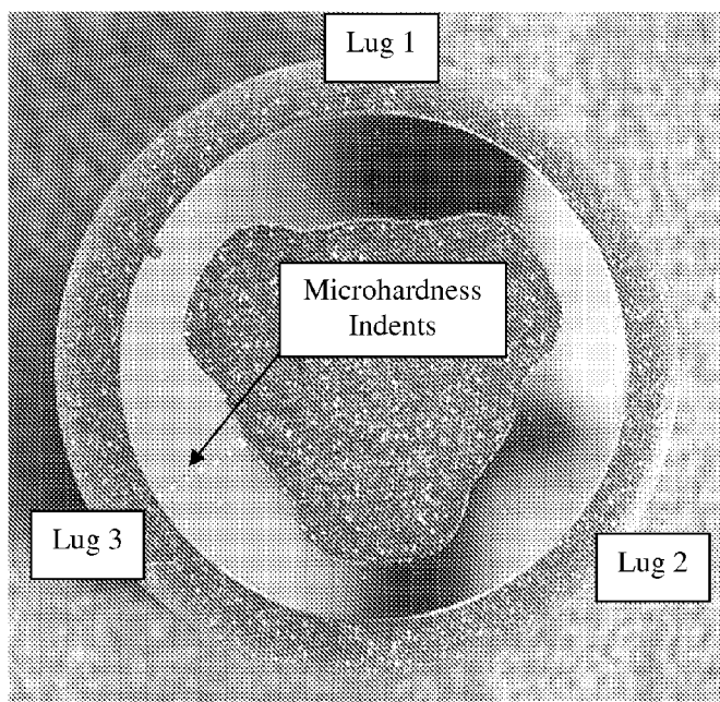
Figure 6: Representative lug section mount.
