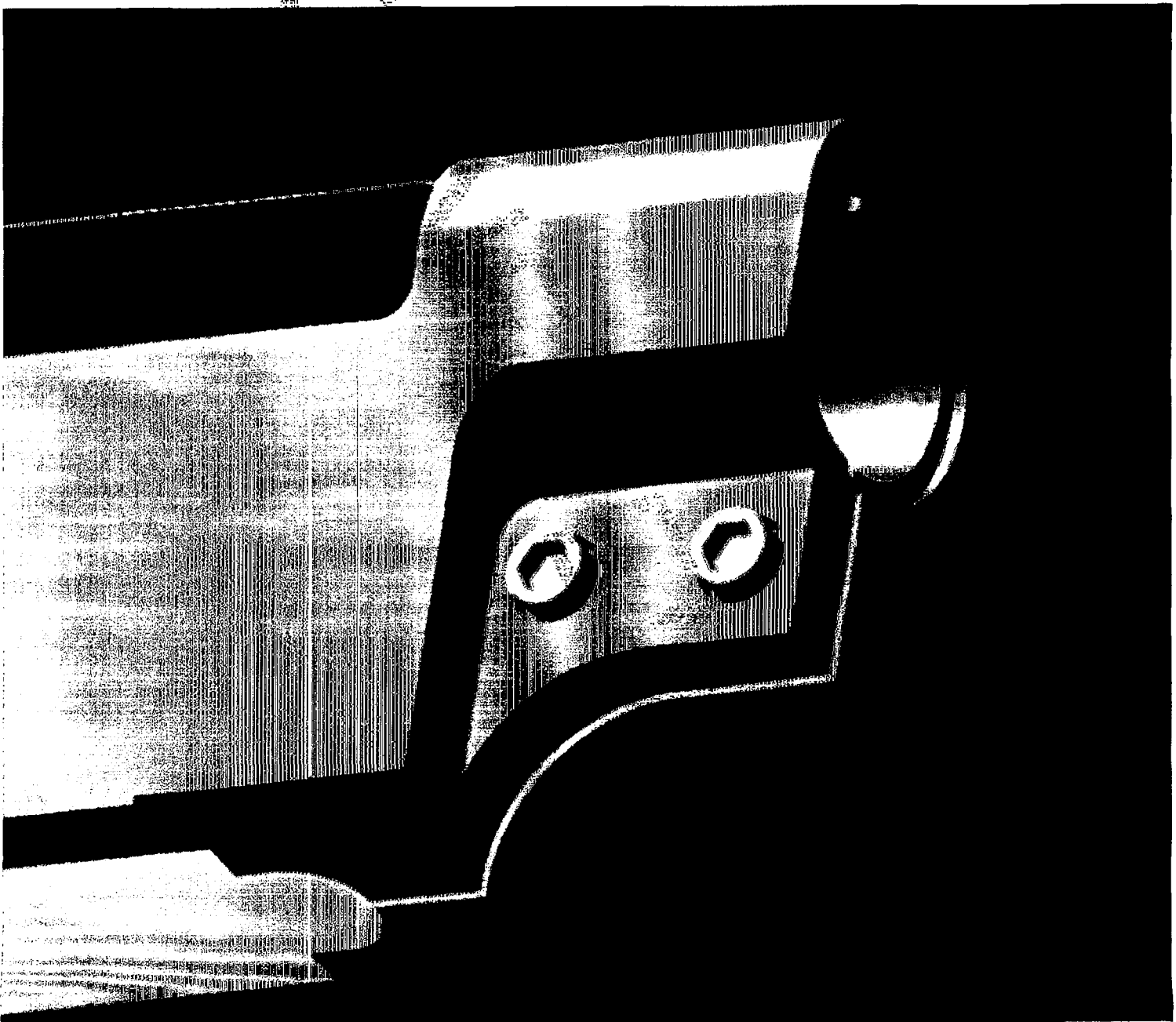
Figure 3. Investment Cast Receiver with Barrel Clamp
