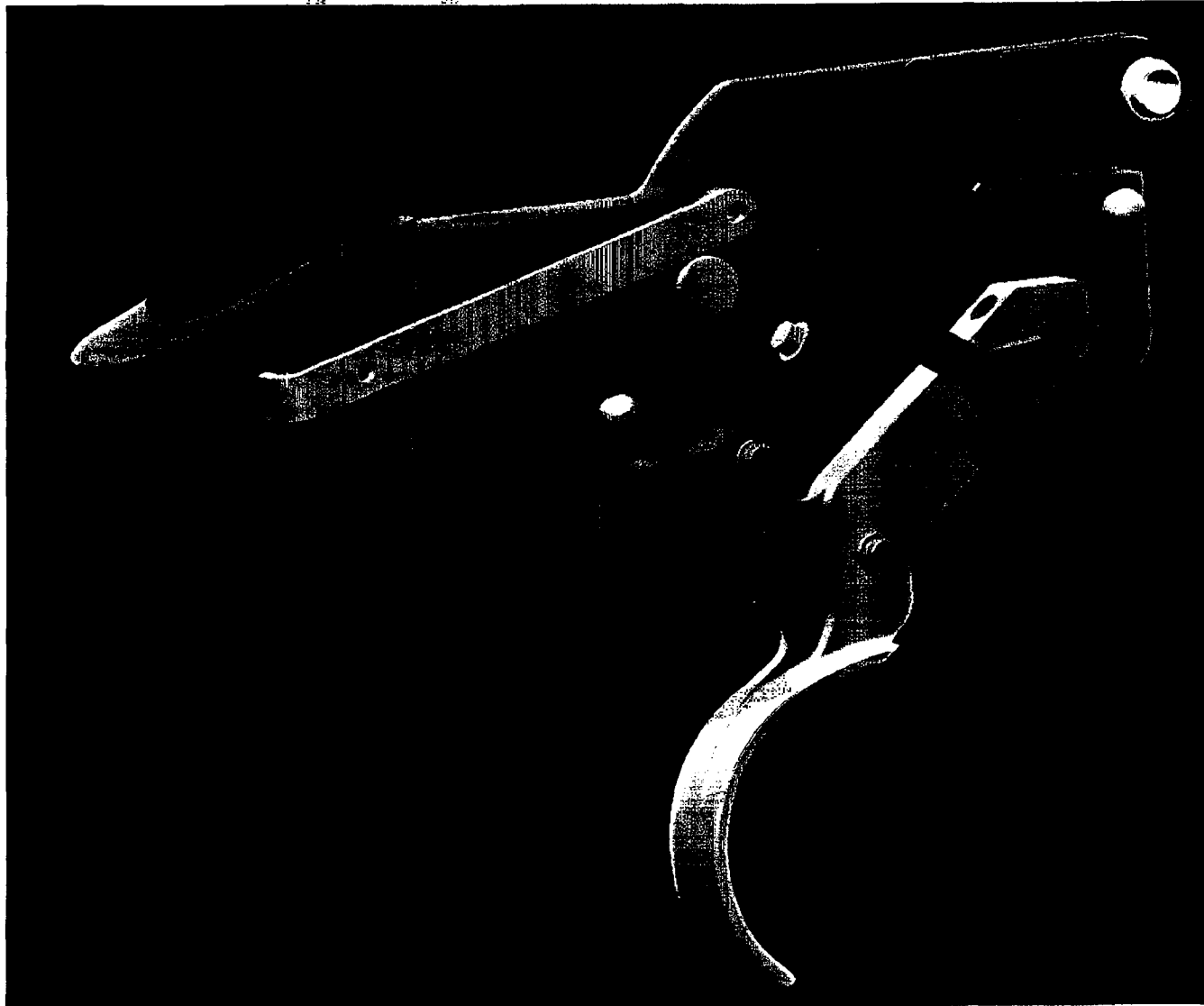
Figure 8. M710 Fire Control Cutaway
