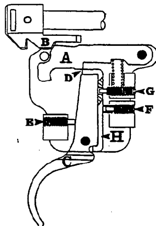
Figure 7 In this commercial override trigger, sear A blocks cocking piece B and is supported by trigger piece C. Engagement of the cocking piece can be large, with sear engagement D small. This trigger is fully adjustable for engagement E, weight F, and overtravel G. Typical weight is two to four pounds, engagement 0.012 inch, overtravel 0.005 inch. Connector strap H between sear A and trigger piece C gives this Remington Model 700 trigger a special "resilient" release, as explained in Rifle 64, page 18.
