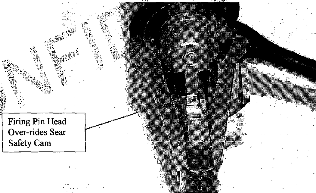
Fig. 3 – Model 710 Over-ride
