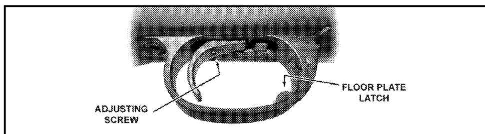
Figure D-5. Adjustment of trigger pull.
