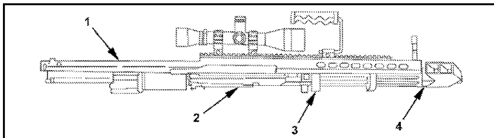
Figure G-19. Extending the barrel.
