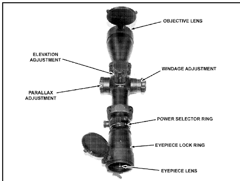
Figure 2-18. Components of the variable scope.
