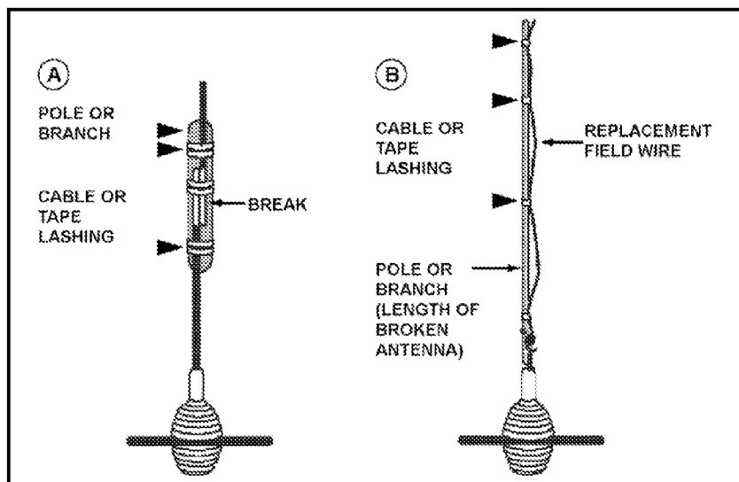
Figure E-10. Repair procedure, whip antenna.
