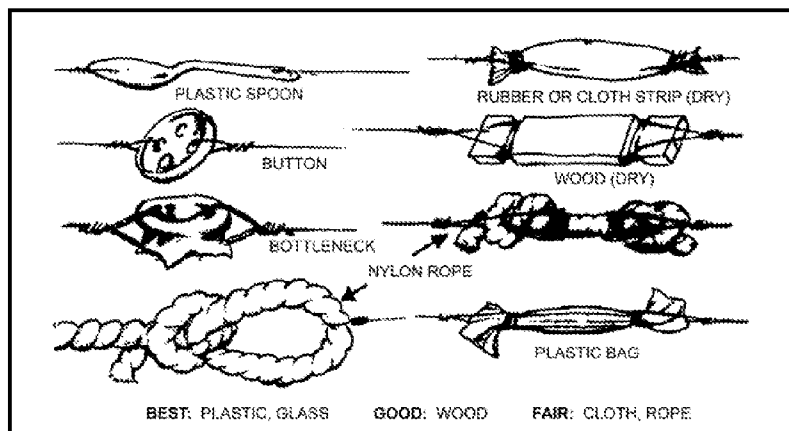
Figure E-9. Expedient Insulators.
