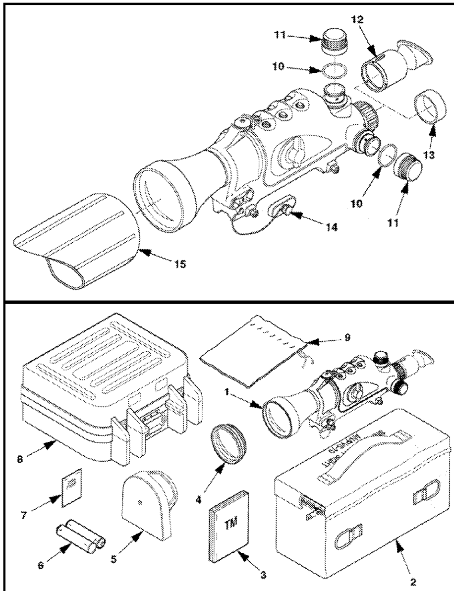
Figure D-14. AN/PVS-10 sniper night scope.
