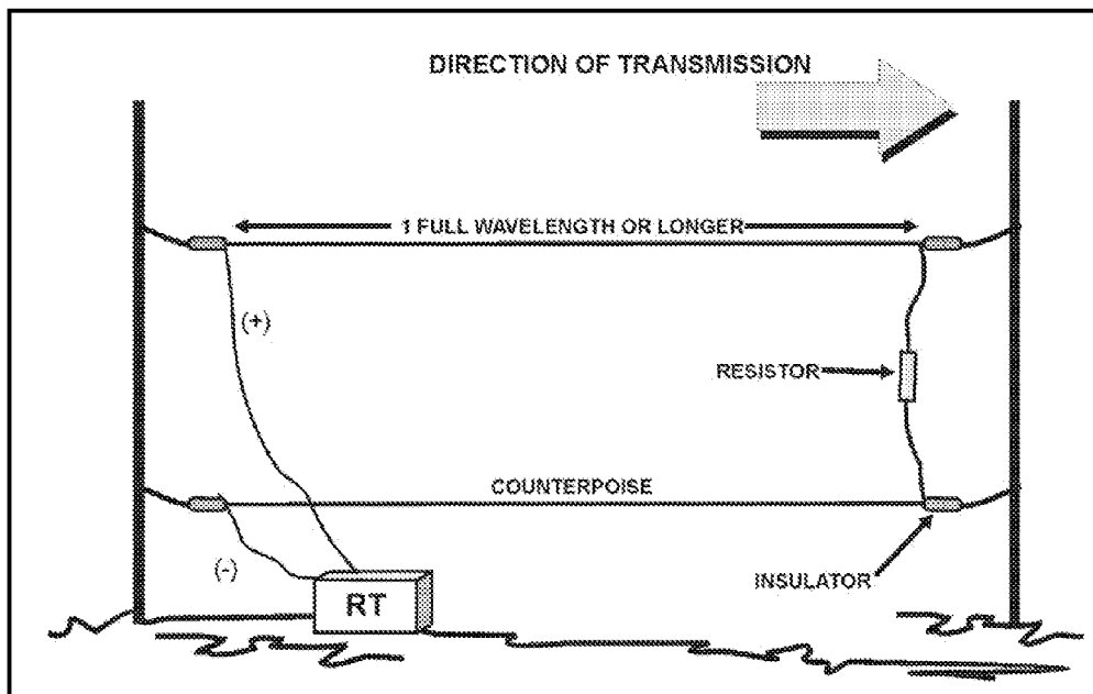
Figure E-6. Long-wire antenna.
