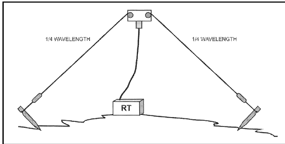
Figure E-5. Inverted "V" antenna.
