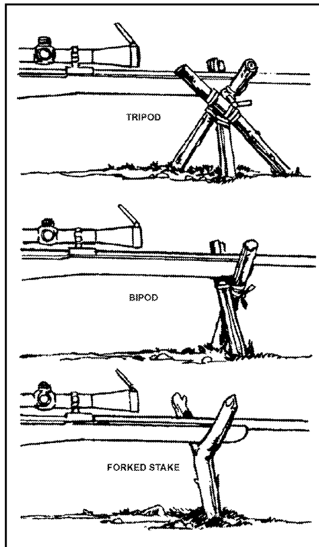
Figure 4-12. Field-expedient tripod, bipod, and forked stake.
