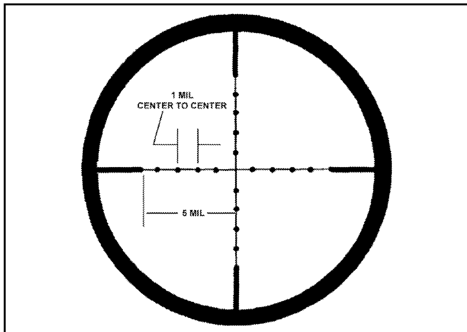
Figure D-13. Mil-dot reticle.
