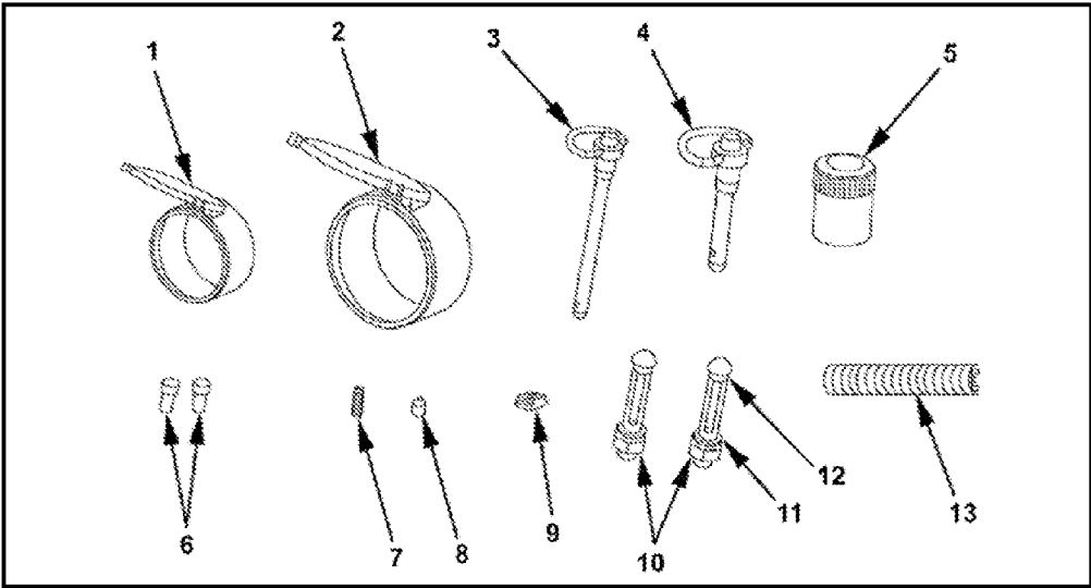
Figure G-25. Deployment parts kit.
