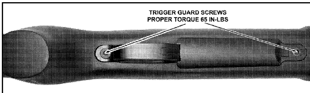
Figure G-29. Trigger guard screws.
