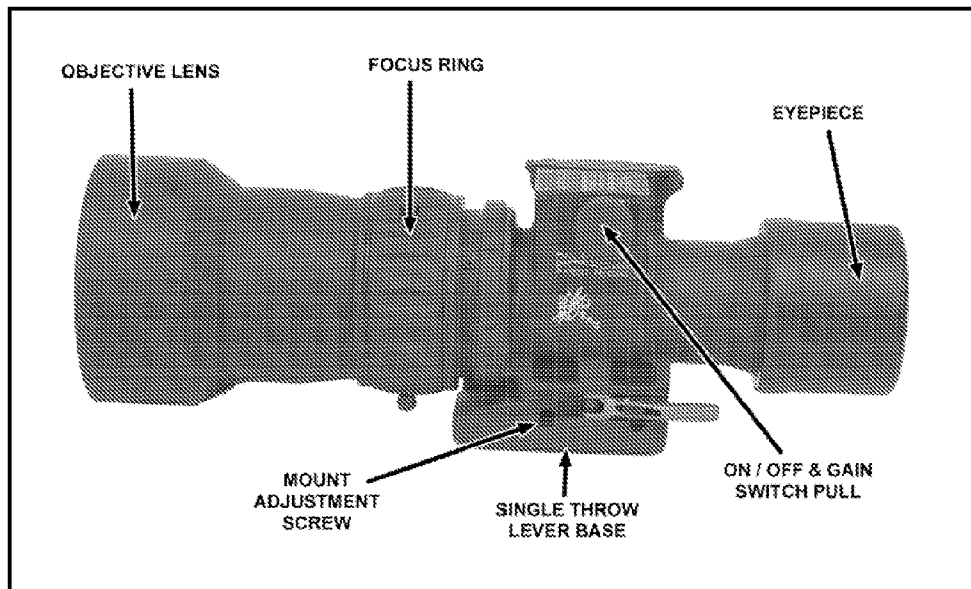
Figure 2-13. AN/PVS-26 universal night sight (left side).
