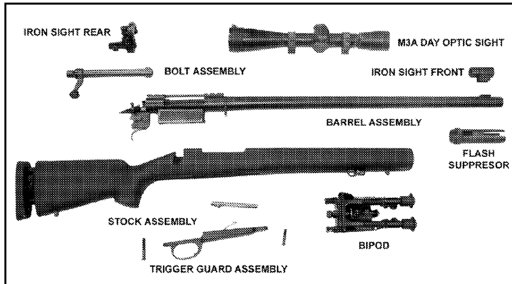
Figure G-27. M24 Sniper Weapon System.
