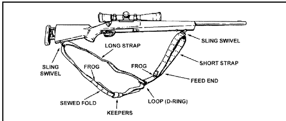
Figure D-7. Sling.
