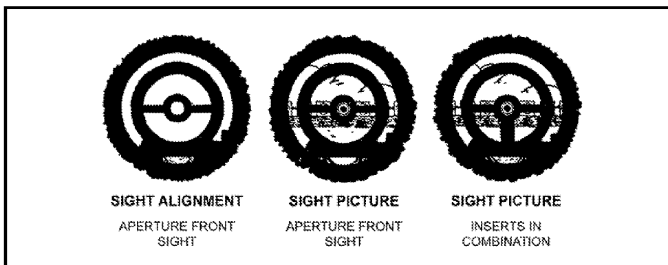
Figure D-19. Aperture insert.
