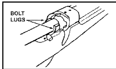
Figure D-4. Alignment of bolt.
