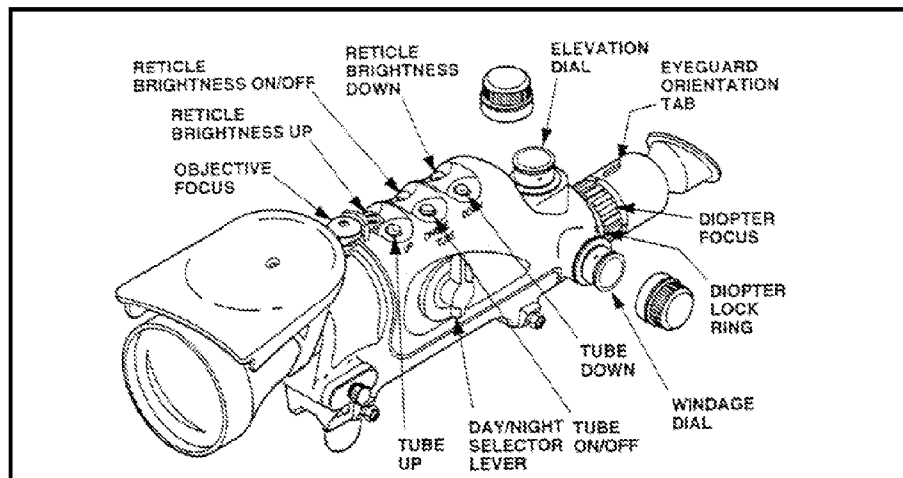
Figure D-16. Controls and indicators.
