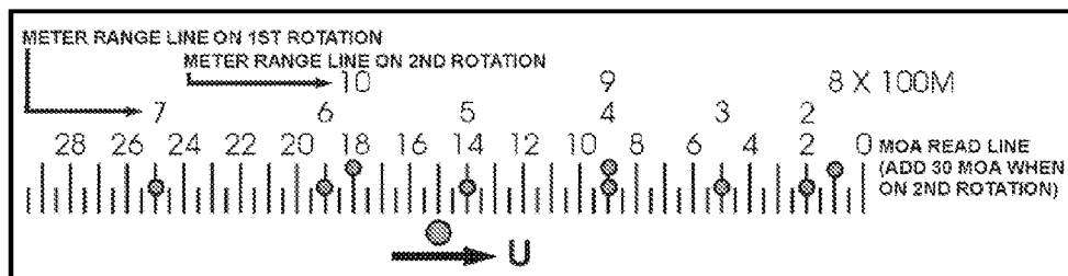
Figure 2-10. Bullet drop compensator.
