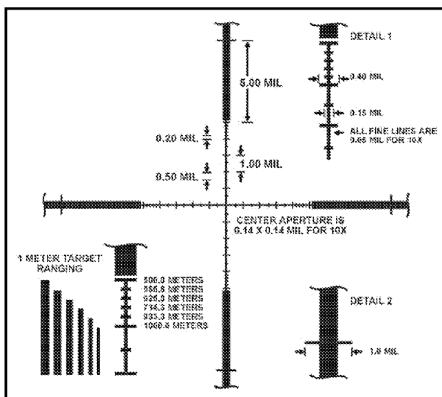
Figure 3-16. Tactical miling reticle breakdown.
