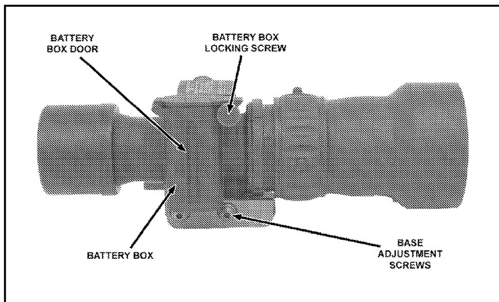
Figure 2-14. AN/PVS-26 universal night sight (right side).
