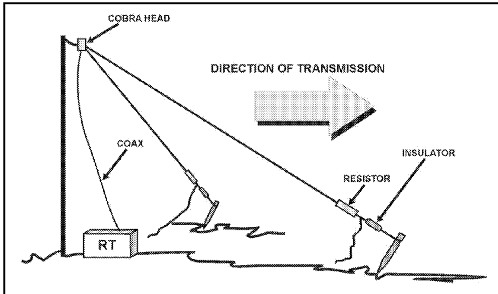
Figure E-8. Terminated sloping "V" antenna.
