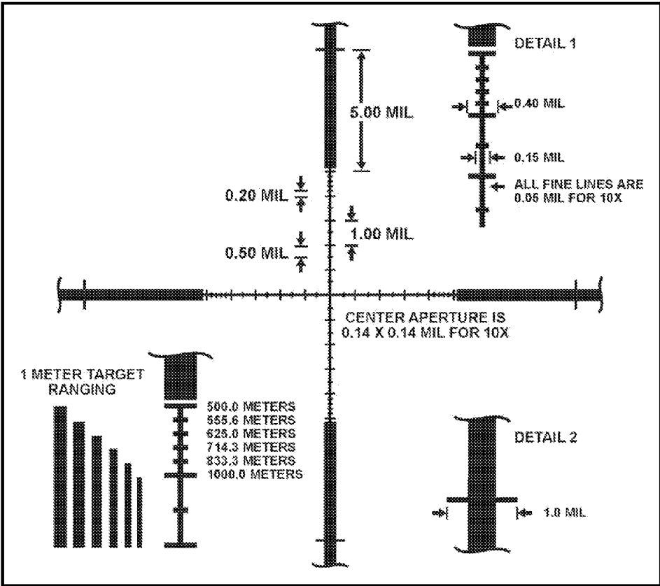
Figure 2-12. Tactical milling reticle breakdown.
