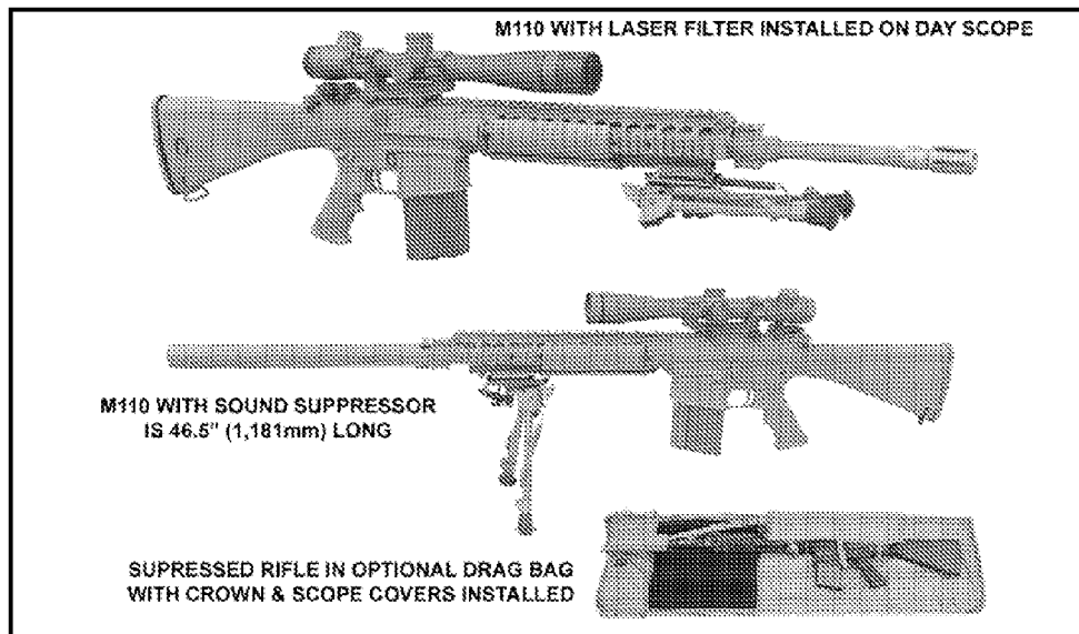
Figure 2-1. M110 Semiautomatic Sniper System.
