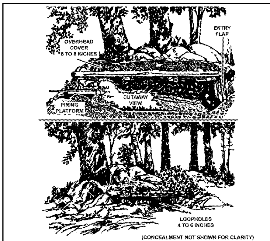
Figure 3-10. Belly hide position.
