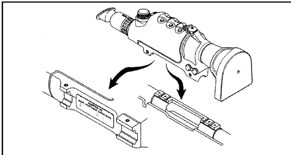
Figure D-17. Mounting base.
