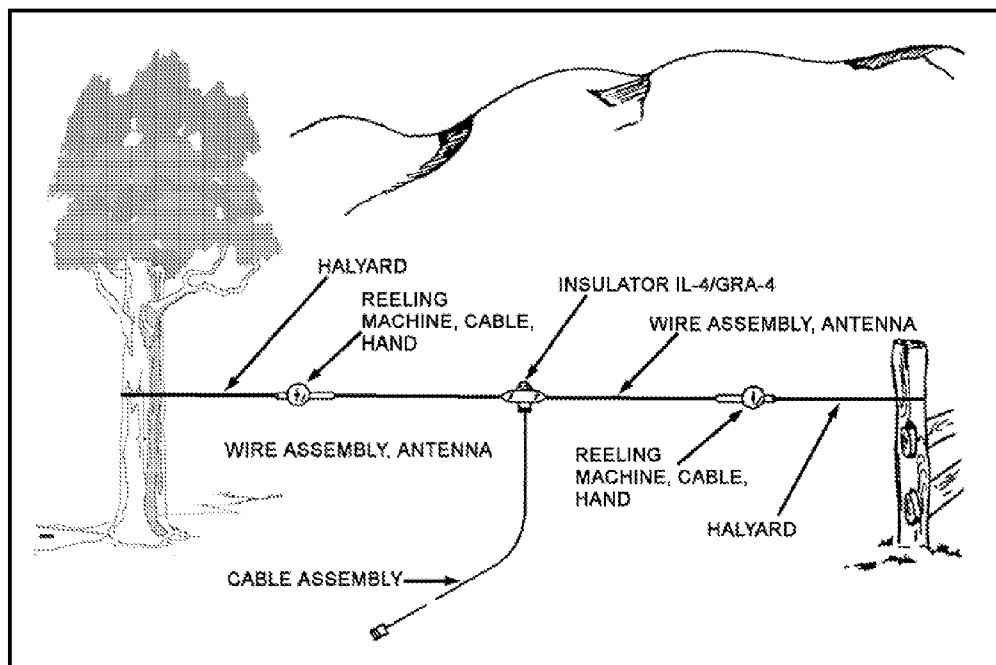
Figure E-4. Half-wave dipole antenna.
