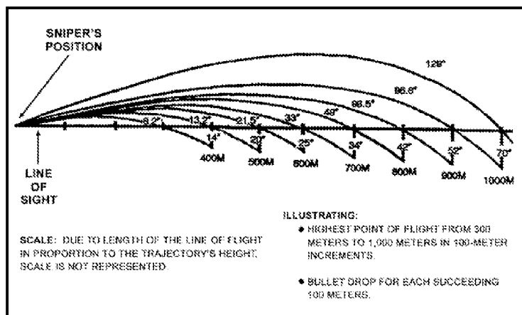
Figure 4-25. Trajectory chart.
