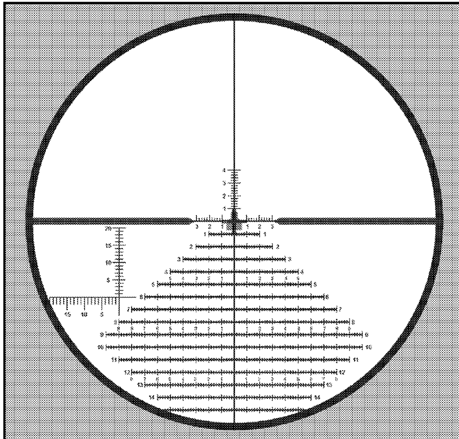
Figure 3-18. Hours H25 mil reticle pattern breakdown.
