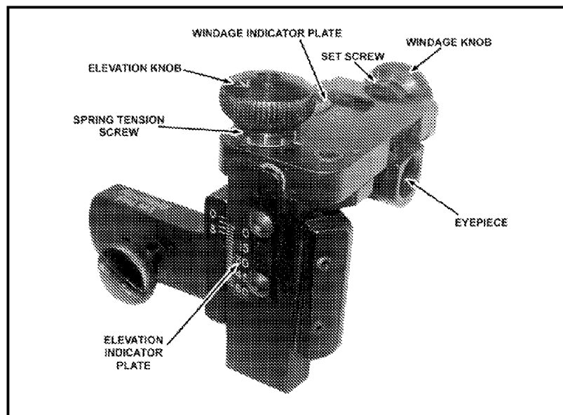
Figure D-21. Zero adjustment dials, iron sights.
