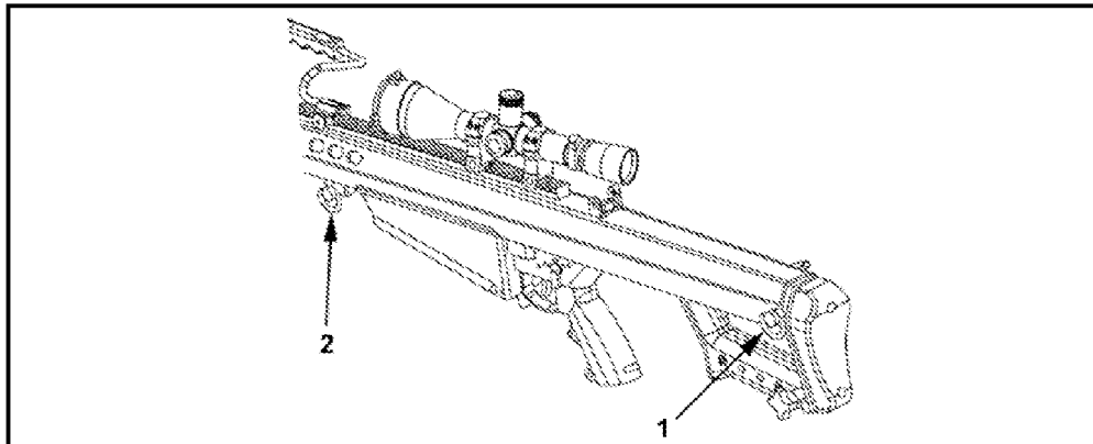
Figure G-5. Rear lock and midlock pins.
