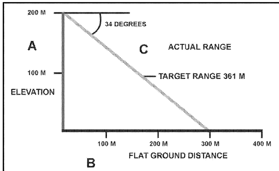
Figure 4-20. Pythagorean Theorem.
